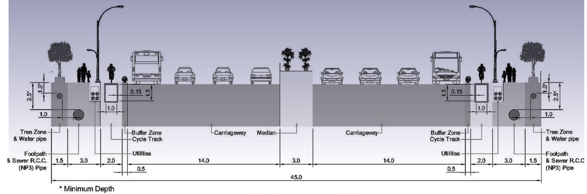
45 M WIDE ROAD CROSS SECTION
