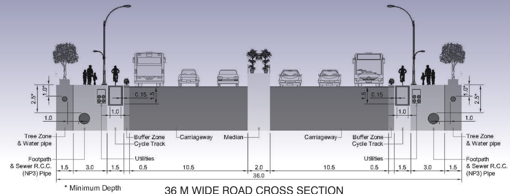
36 M WIDE ROAD CROSS SECTION
